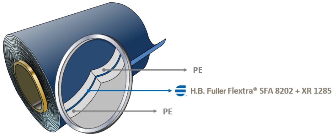
Figure 1. 'Flextra® SFA 8202 + XR 1285' technology by H.B. Fuller used as laminating adhesive.
