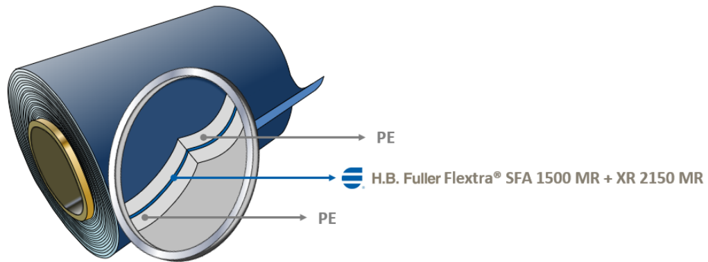
Figure 1. 'Flextra® SFA 1500 MR + XR 2150 MR' technology by H.B. Fuller used as laminating adhesive.
