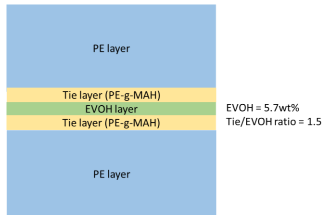
Figure 1. 'PE/EVOH barrier with PE-g-MAH' technology by Kuraray.
