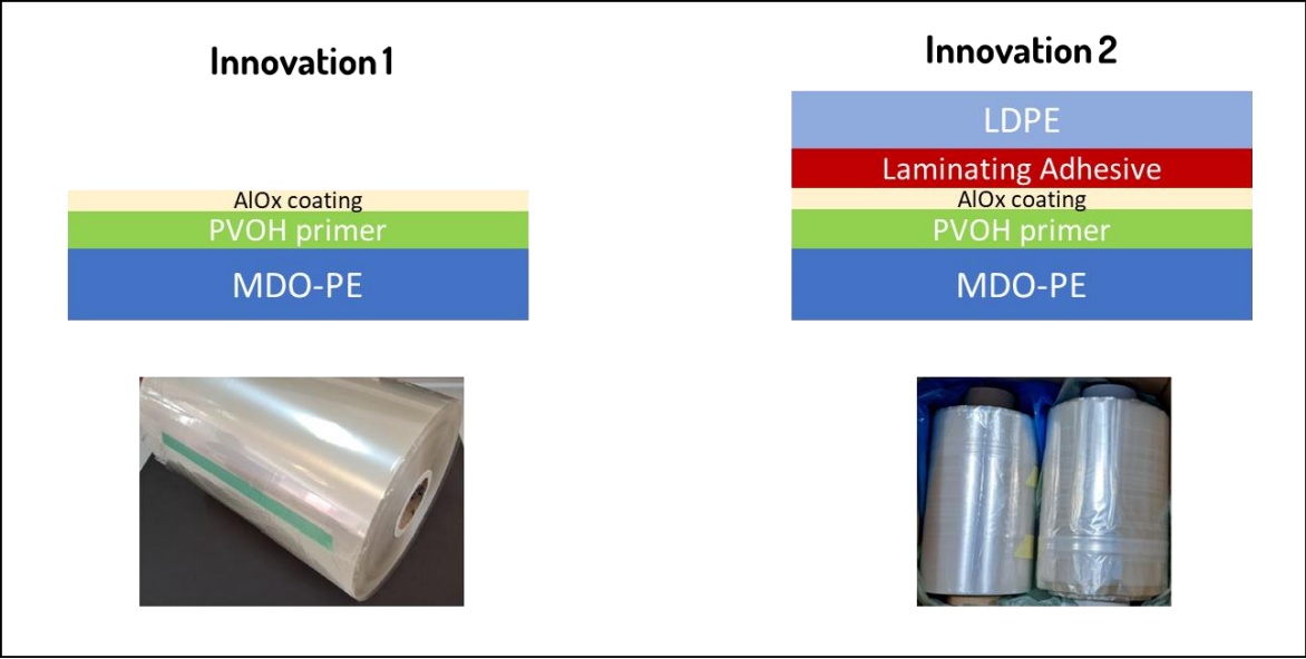
Figure 1: Composition of samples used for the test campaign.
