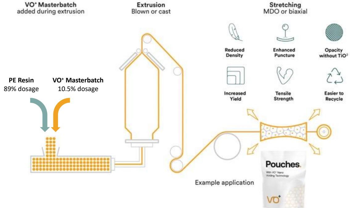
Figure 1 'VO+ PE 1300 Series Voiding Agent' technology by VOID Technologies
